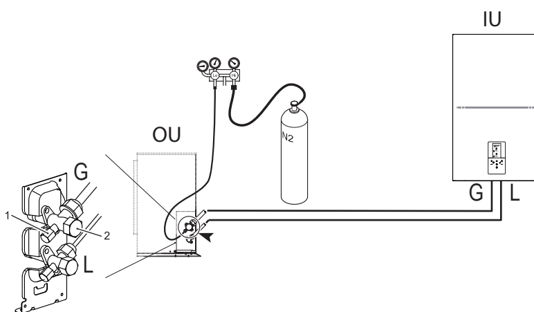
fig. 12 - Airtight test and leakage detection
