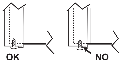
fig. 15 - assembly with bottom screws
