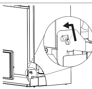
fig. 18 - how to release the electric box
