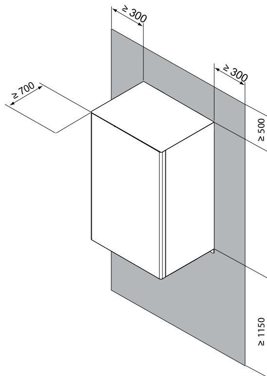
fig. 7 - minimum operating area for indoor unit
