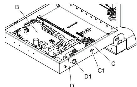
fig. 20 - Internal view of electrical cabinet
