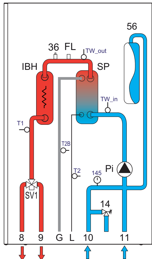
fig. 5 - Indoor unit hydraulic diagram
